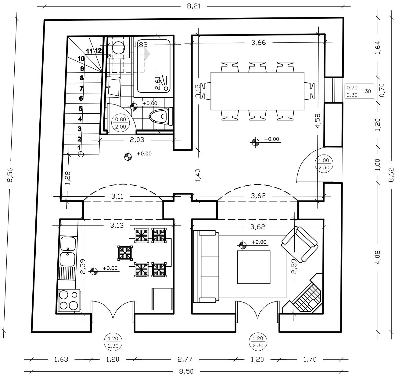
GROUND FLOOR PLAN VIEW COVERED AREA: 71,75 M2
